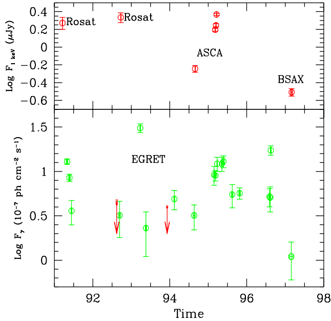
Fig. 4. Historical light curves in the X-ray and \gamma -ray bands, after 1991. All X-ray data have been reanalysed assuming a fixed N_{\text{H}} = 5.3 \times 10^{21} \text{ cm}^{-2} .
